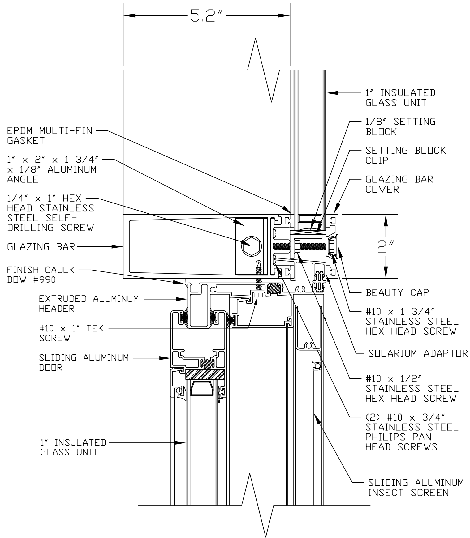
SLIDING DOOR HEAD DETAIL
