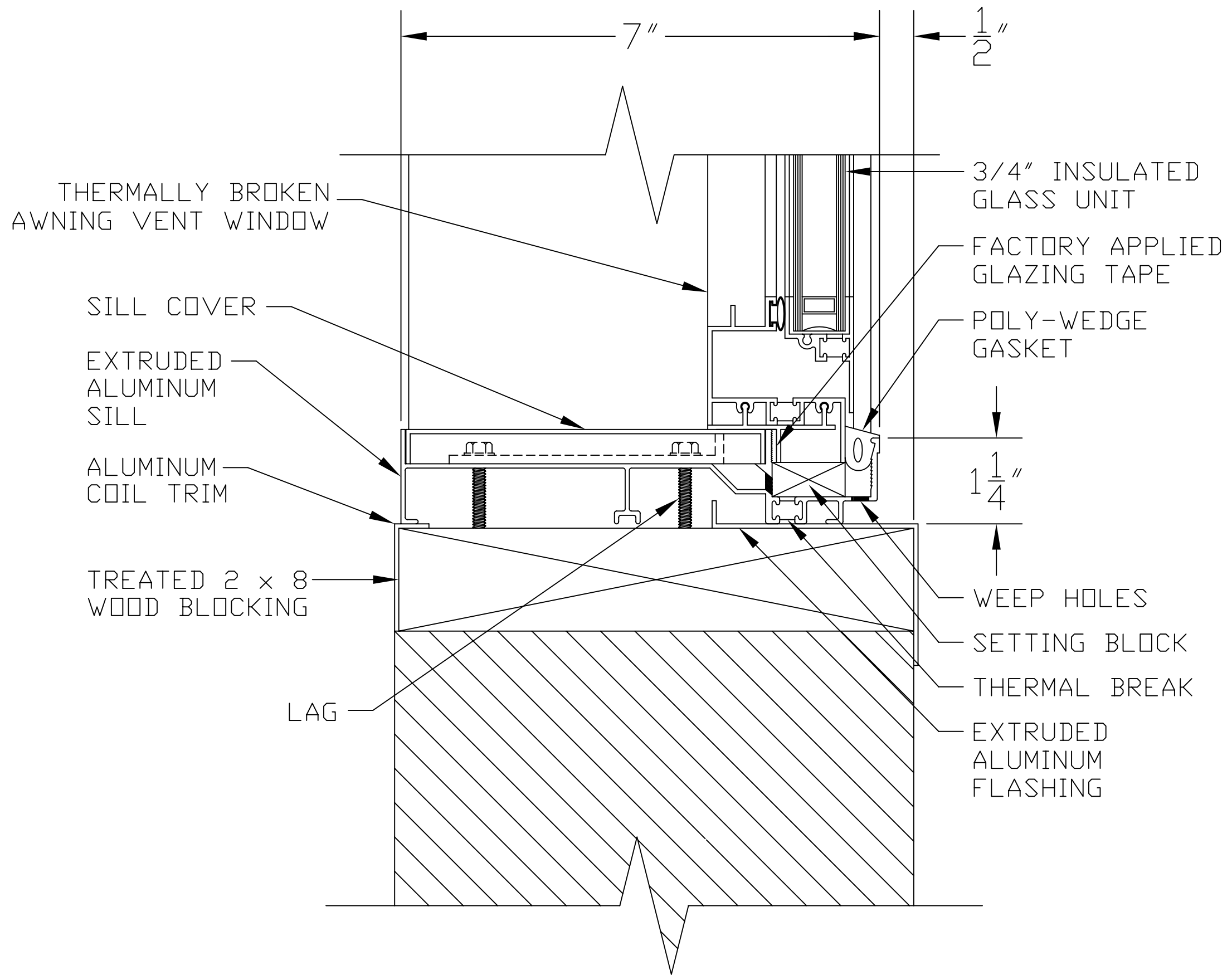
AWNING WINDOW SILL DETAIL
